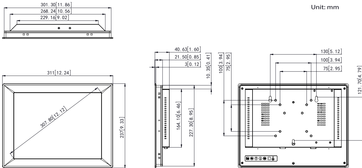
Panel Cut-out Dimensions: FPM-2120G 303.3 x 229.3 mm (11.94" x 9.03")
