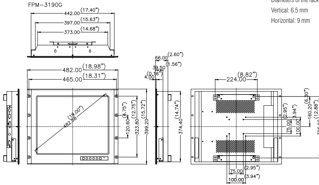
Cut out dimension 444x376.4mm (17.48"x14.81")
