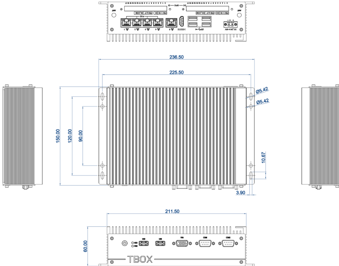
DIMENSIONAL DRAWING:TBOX-3TX0/3DX0
