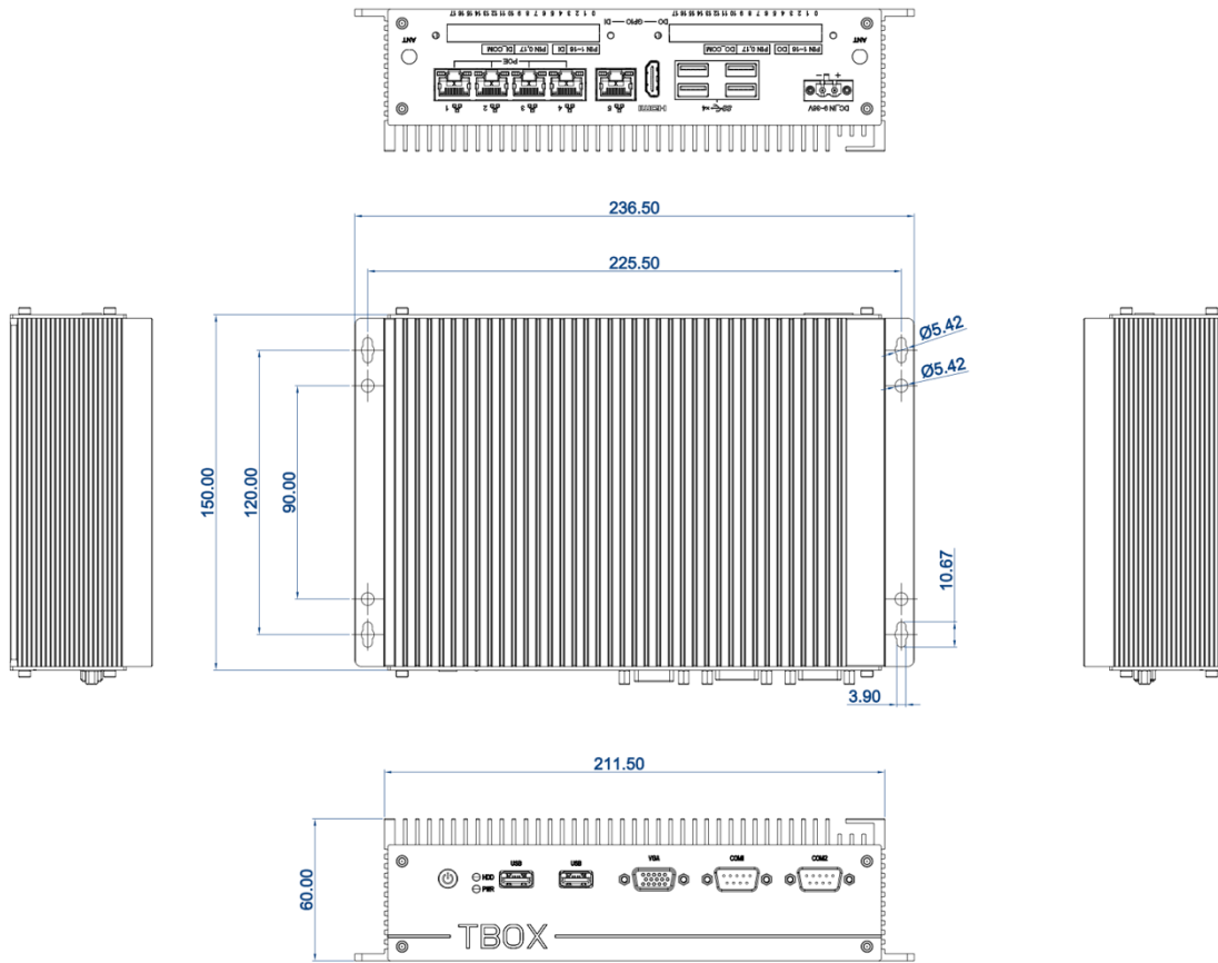
DIMENSIONAL DRAWING:TBOX-3TX0/3DX0
