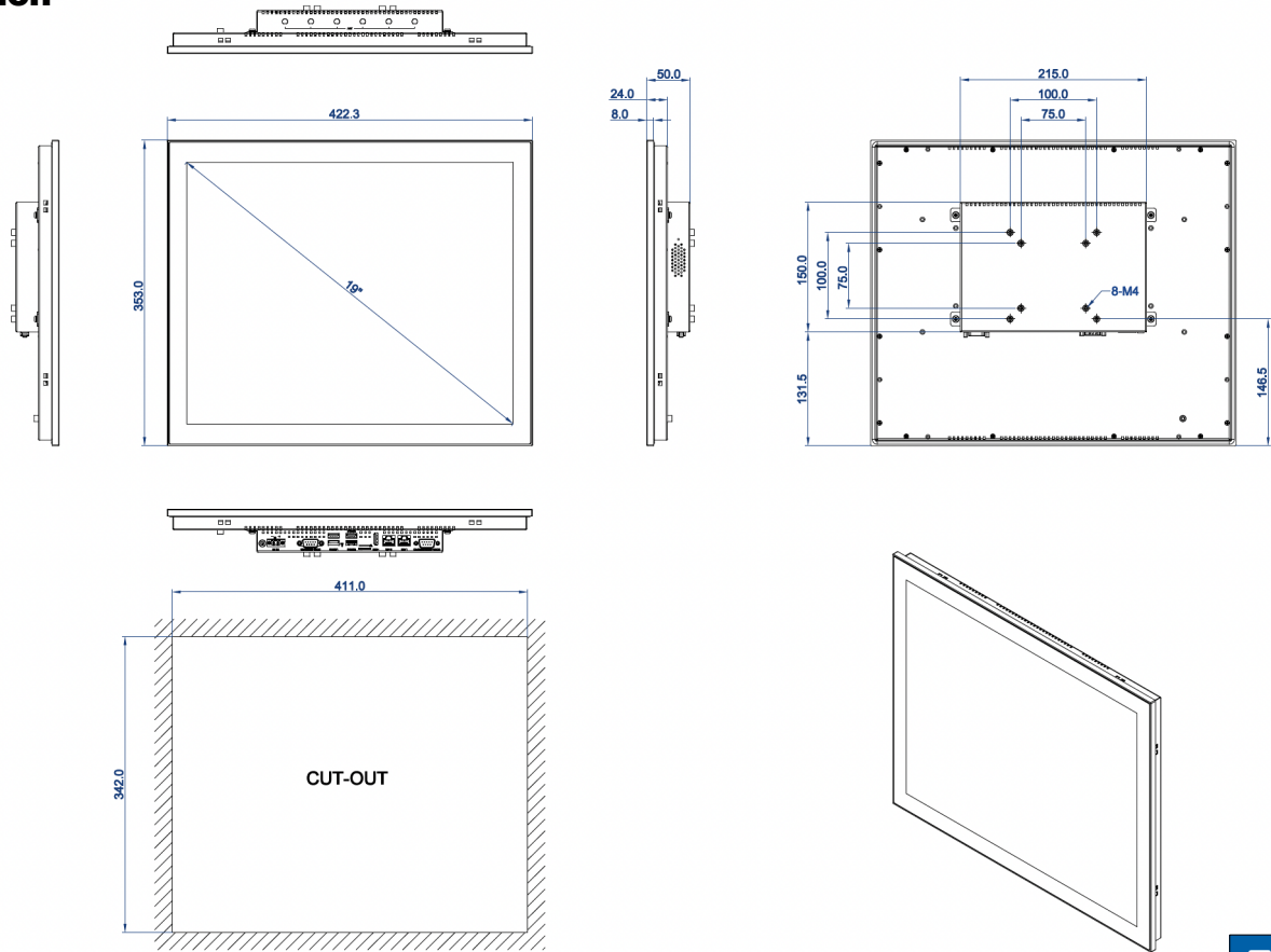
DIMENSIONAL DRAWING:TPC-DCS190R2
